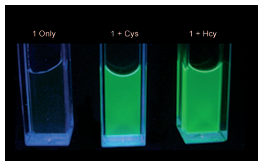
Figure 2. A photograph showing the fluorescence emission of 1 when treated with Cys or Hcy.
