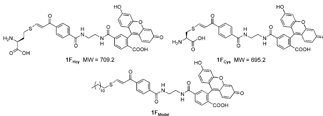
Scheme 4. Structures of the fluorescent parts 1F Hcy , 1F Cys and 1F Model .
