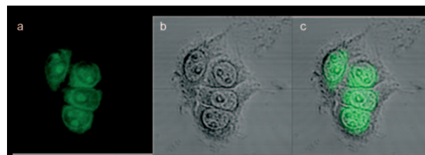
Figure 8. Fluorescence and brightfield images of fixed SK-HEP-1 cells: a) fluorescence image of cells incubated with 1 ( 10\text{ }\mu\text{M} ) for 10 min at room temperature; b) brightfield image of cells shown in panel a; c) the overlay of panels a and b.
