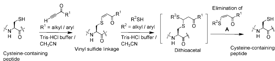
Scheme 1. Electron-deficient alkynes as cleavable reagents for modification of cysteine-containing peptides in aqueous medium.
