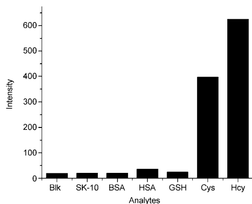
Figure 4. Enhancement of emission intensity of 1 by SK-10, BSA, HSA, GSH, Cys and Hcy.
