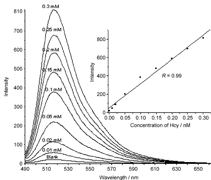
Figure 3. Emission spectral traces of 1 (5 \mu M) in PBS buffer with increasing [Hcy]/[ 1 ] ratio (from 0 to 60) at room temperature. Each spectrum was acquired 15 min after Hcy addition.
