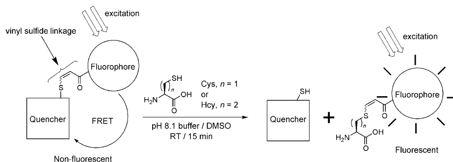
Scheme 2. Turn-on fluorescence can be achieved after removal of the quencher by the thiol-assisted cleavage of the vinyl sulfide linkage.
