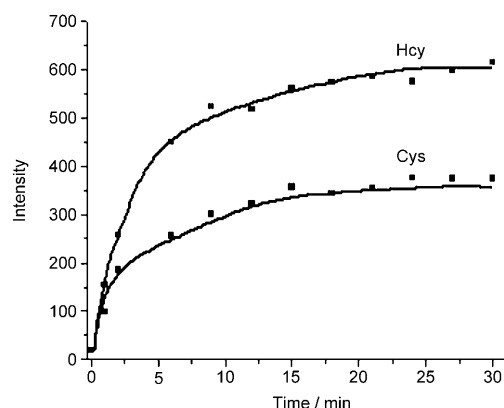
Figure 1. Respective time course of the reaction between 1 and homocysteine and cysteine in a molar ratio of 1:40.
