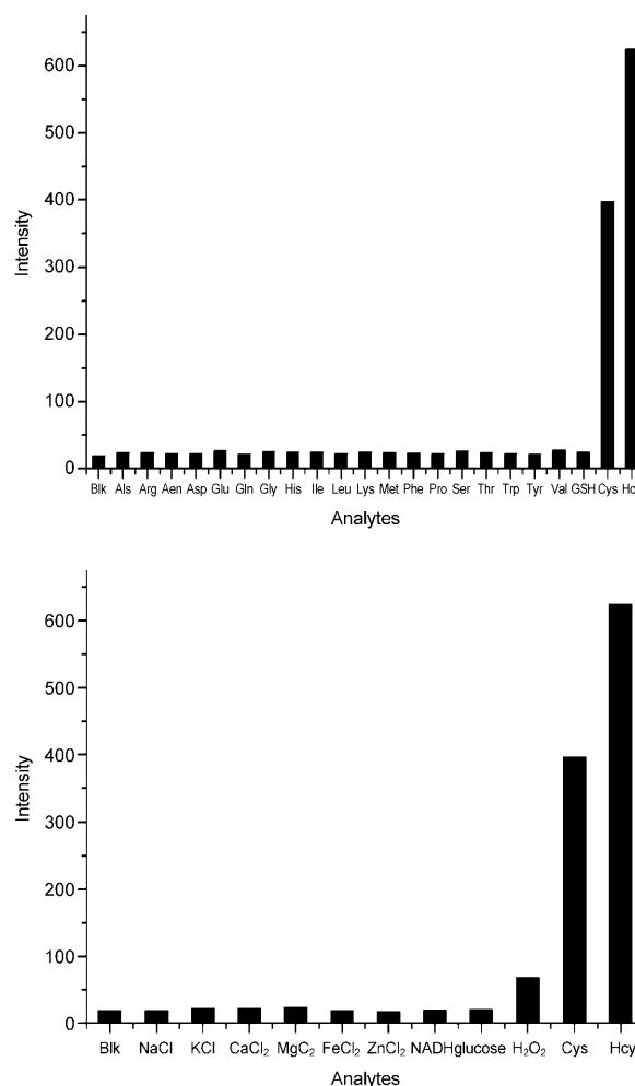
Figure 5. Enhancement of emission intensity of 1 by different analytes.
