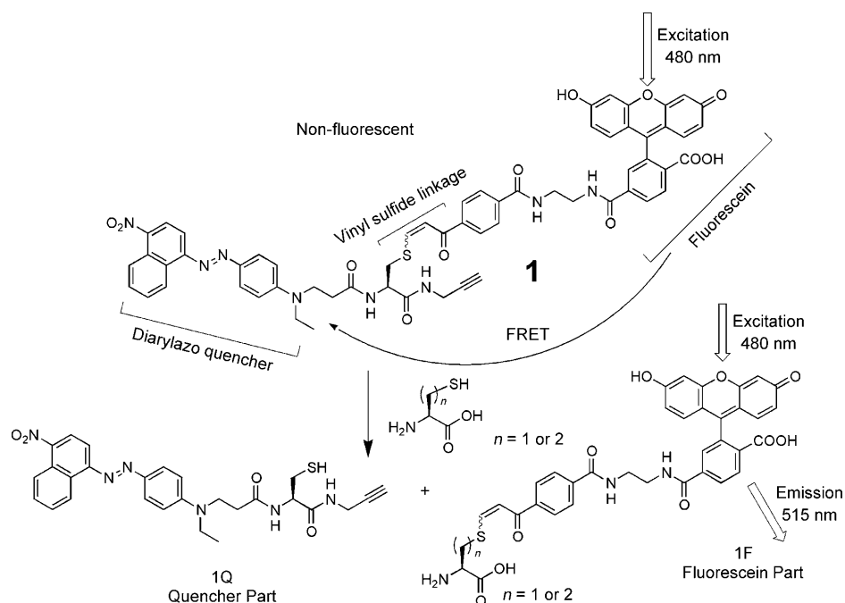
Scheme 3. Working principle of 1 as a fluorescent sensor in response to cysteine and homocysteine.
